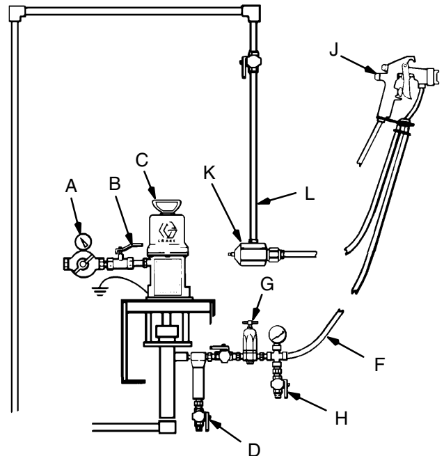
Single Circulating Spray Station
